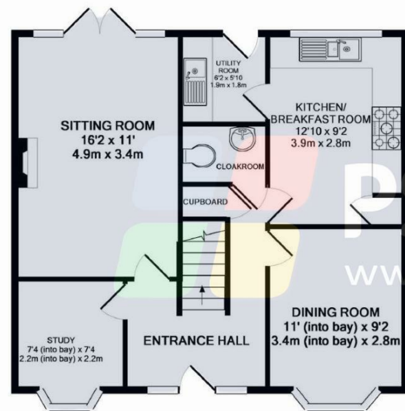
GROUND FLOOR APPROX. FLOOR AREA 626 SQ.FT. (58.1 SQ.M.)
